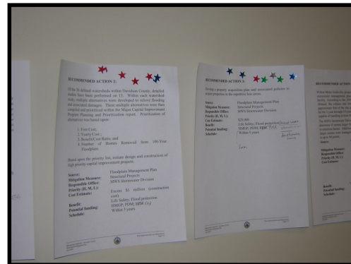
Prioritization “Stars”
