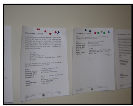
Figure 5.1 Priority “Stars”
